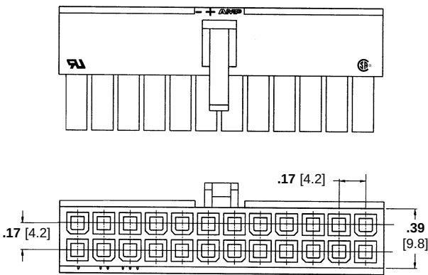
Receptacle Housing
