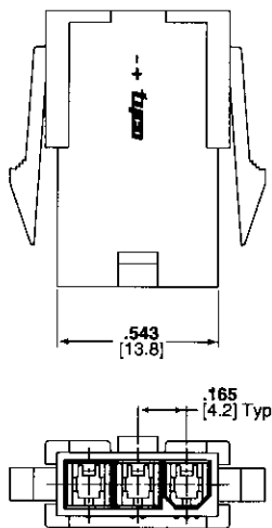
Panel Mount Plug Housing
